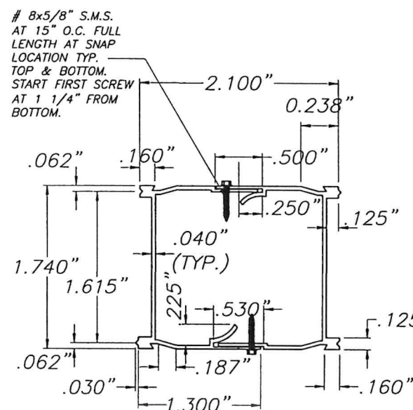
9 MULLION SCALE : 3/4" = 1" 6063-T6 ALUMINUM ALLOY
