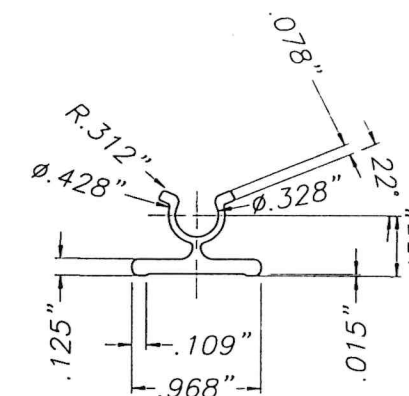
4 MALE HINGE SCALE : 3/4" = 1" 6063-T5 ALUMINUM ALLOY
