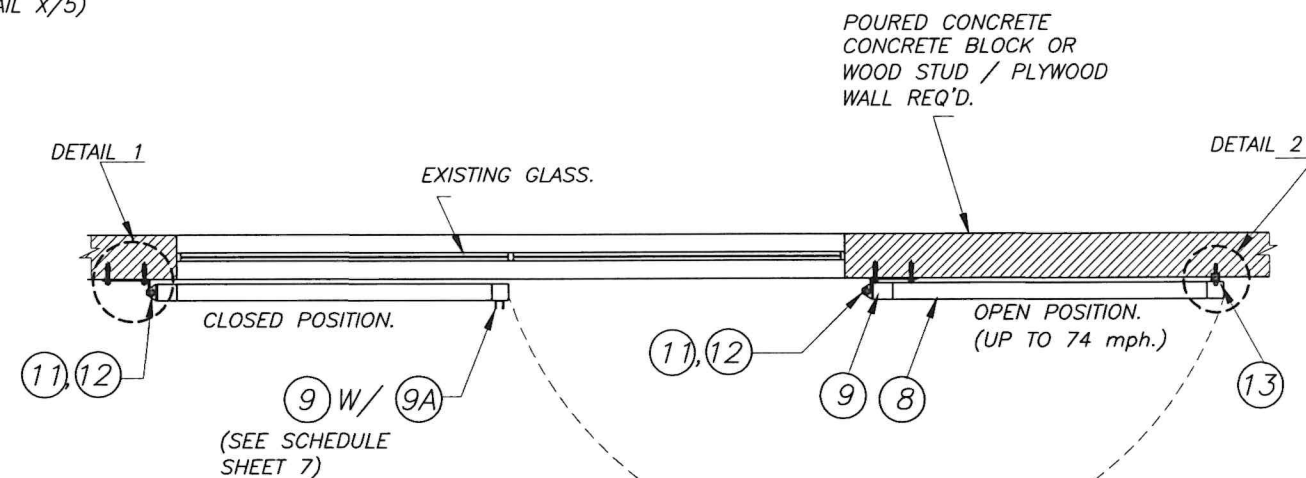
SECTION C-C (OPEN POSITION, UP TO 74 mph. WIND SPEED).
