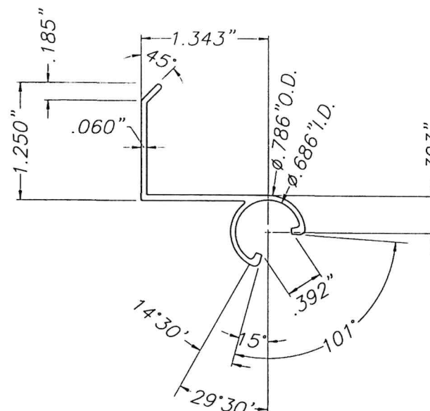
3 AWNING RAIL SCALE : 3/4" = 1" 6063-T6 ALUMINUM ALLOY
