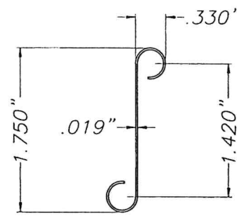
2 ALTERNATE TYPE 2 SLAT SCALE : 3/4" = 1" 3004-H36 ALUMINUM ALLOY ROLL FORM
