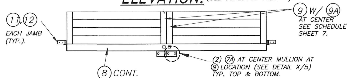
ALTERNATE ELEVATION (CLOSED POSITION) SIMILAR APPLICABLE TO TOP.
