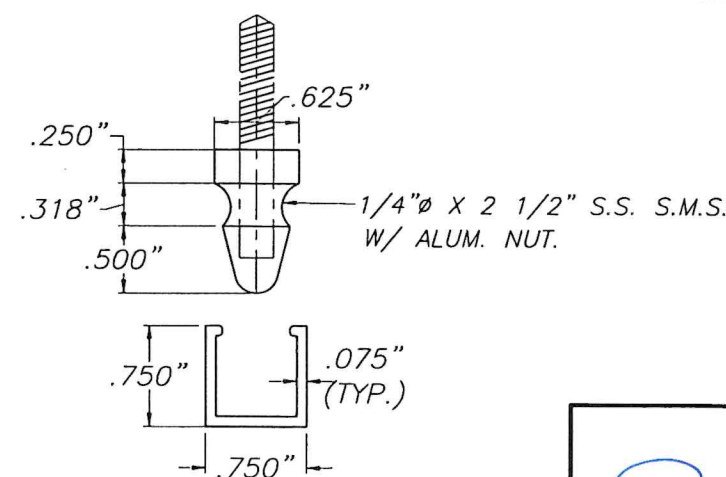
13 HOLD BACK LATH SCALE : 3/4" = 1" 6063-T6 ALUMINUM ALLOY 1" LONG
