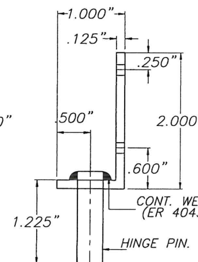
9A MULLION INSERT SCALE : 3/4" = 1" 6063-T6 ALUMINUM ALLOY
