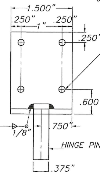
7 & 7A LOCK BRACKET SCALE : 3/4" = 1" 6063-T6 ALUMINUM ALLOY
