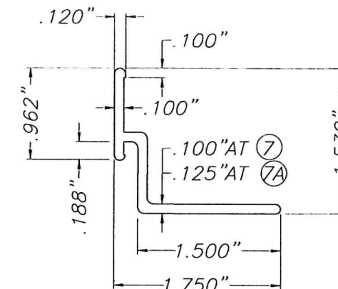
7 = CONTINUOUS 7A = 3" LONG AT END MULLIONS = 3" LONG AT CENTER MULLIONS
