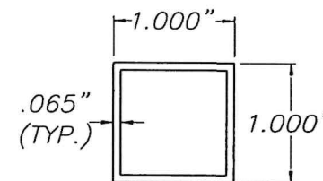
9A MULLION INSERT SCALE : 3/4" = 1" 6063-T6 ALUMINUM ALLOY
