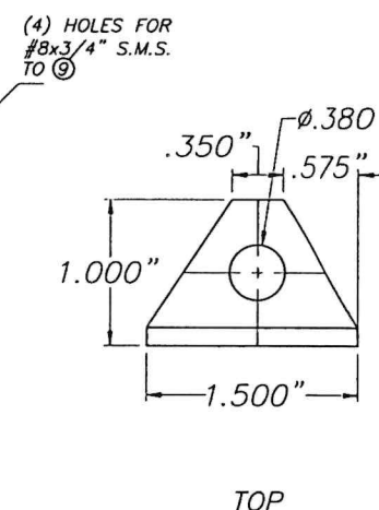
7 & 7A LOCK BRACKET SCALE : 3/4" = 1" 6063-T6 ALUMINUM ALLOY
