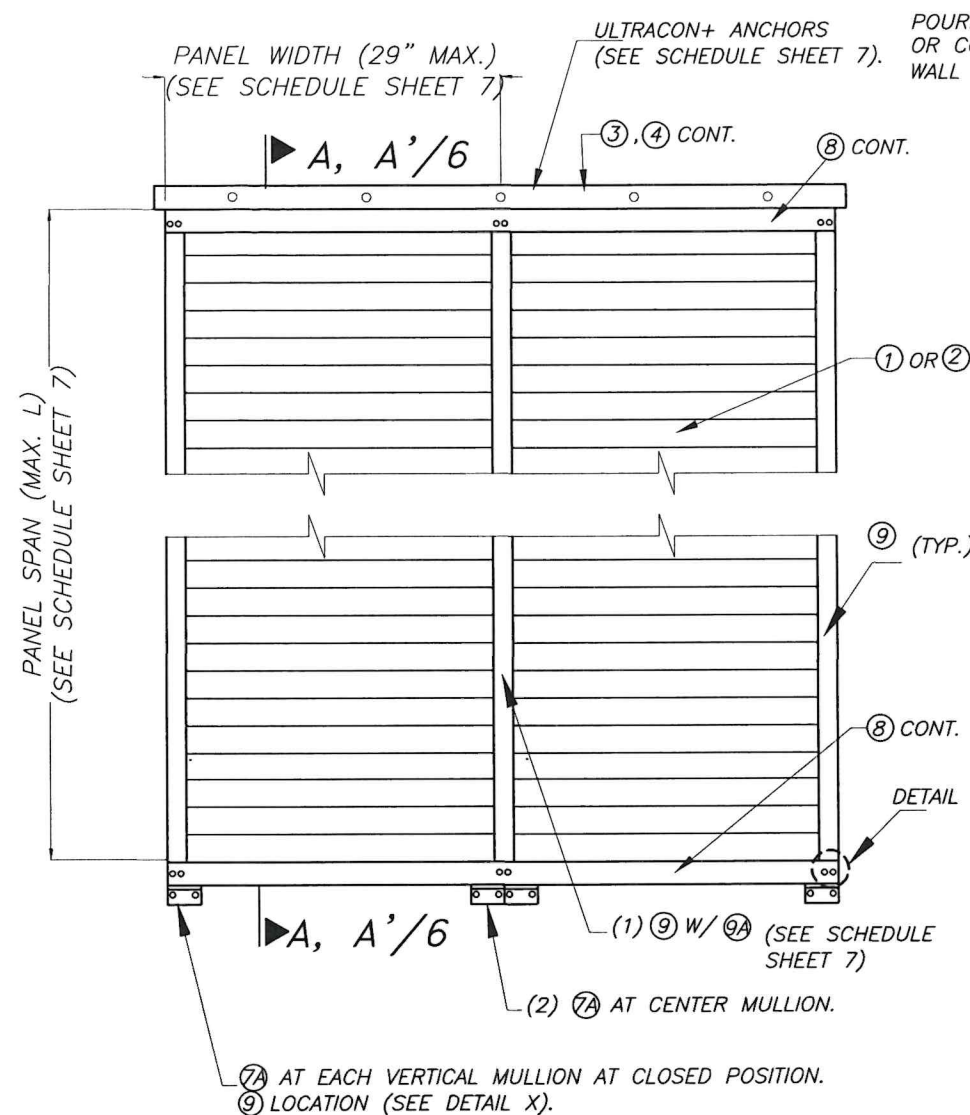
ELEVATION SCALE= 1/2"-1'-0"
