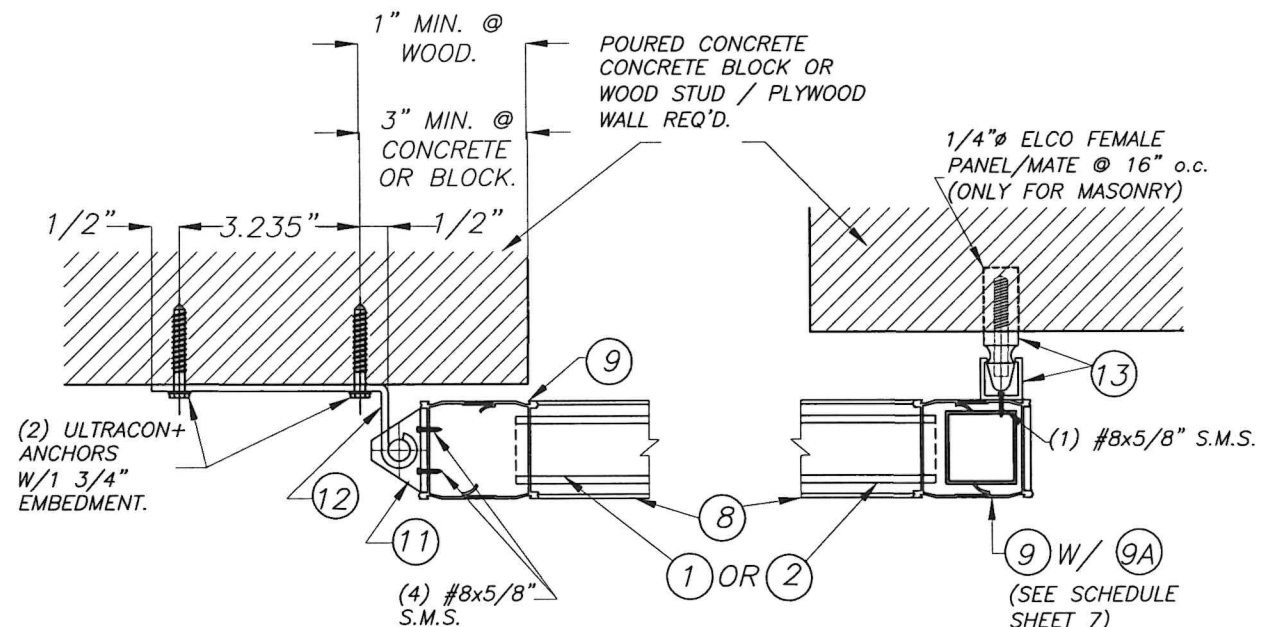
DETAIL 1 (PLAN).
