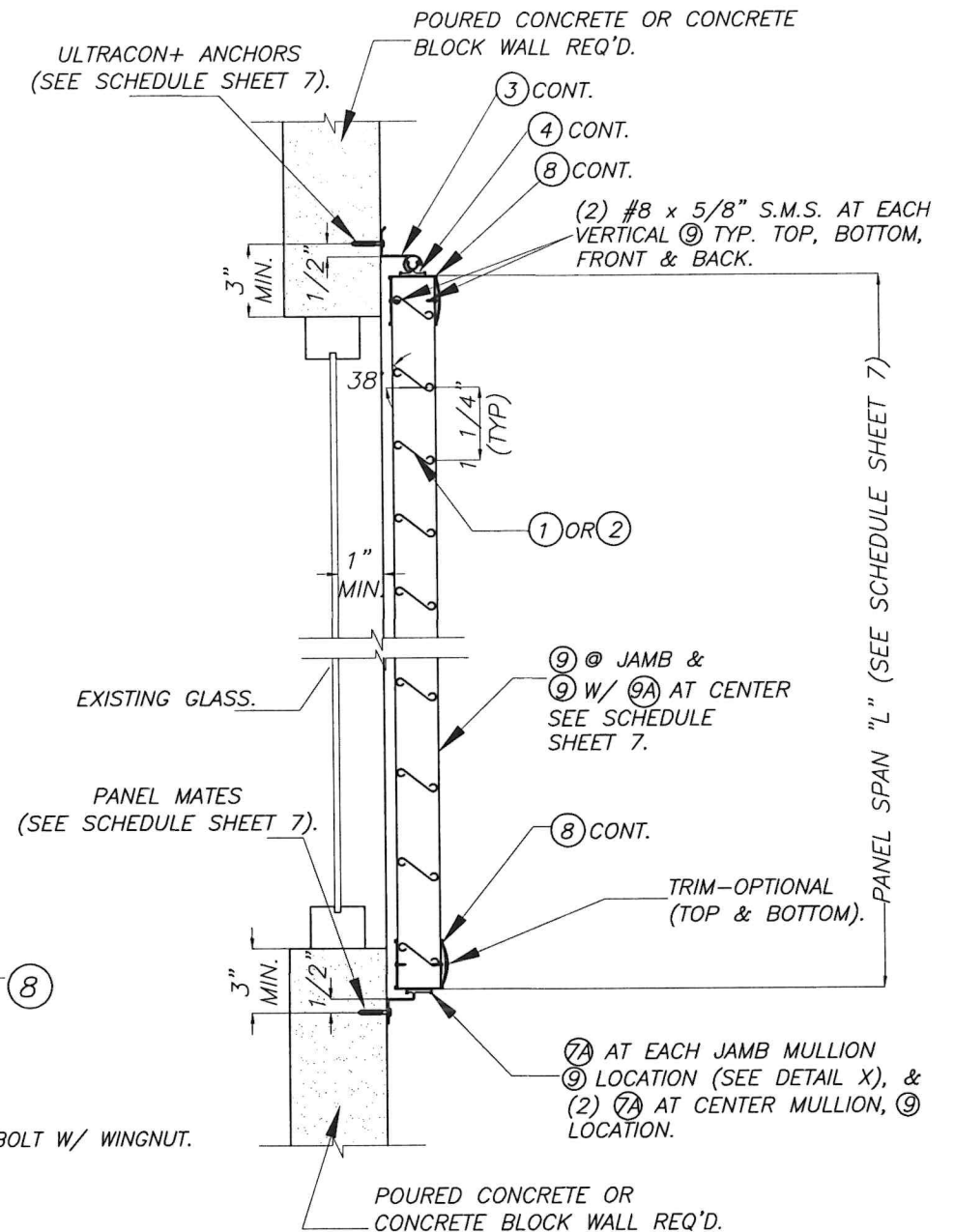
SECTION A-A (CLOSED POSITION). SCALE= N.T.S.
