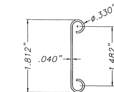
1 TYPE 1 SLAT SCALE : 3/4" = 1" 6063-T5 ALUMINUM ALLOY
